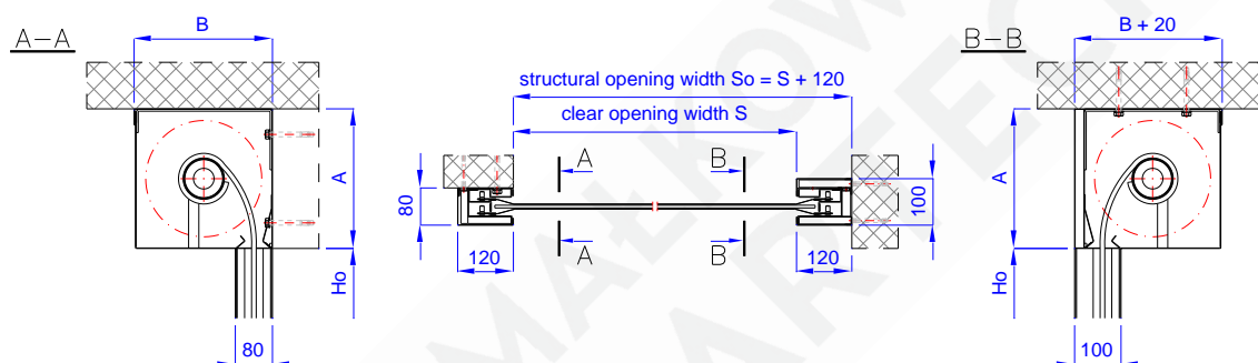
Fig. 3 – Fire protection curtain door MARC-Ok EI60, mixed mounting - no lintel and reveal on the right side
