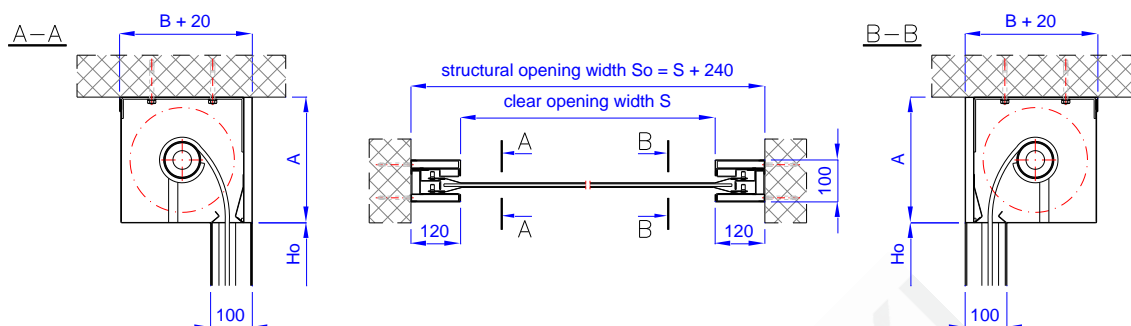
Fig. 2 – Fire protection curtain door MARC-Ok EI60, corridor (niche) mounting - no lintel and both reveal
