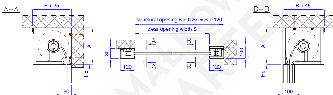
Fig. 3 – Fire protection curtain door MARC-Ok EI90, mixed mounting - no lintel and reveal on the right side
