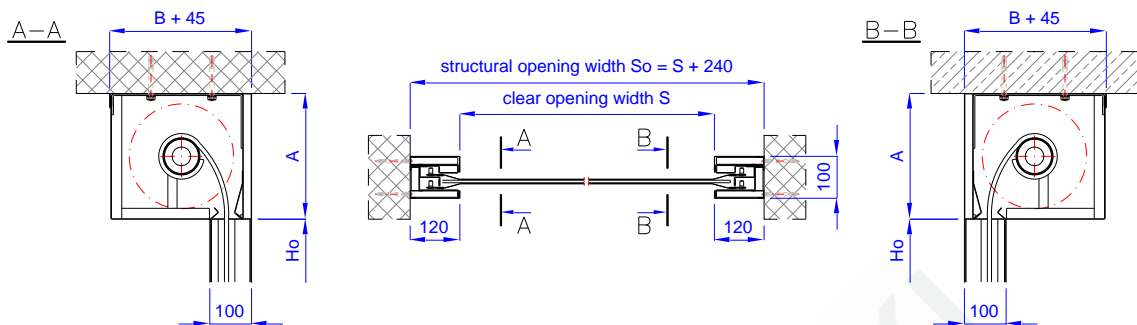
Fig. 2 – Fire protection curtain door MARC-Ok EI90, corridor (niche) mounting - no lintel and both reveal
