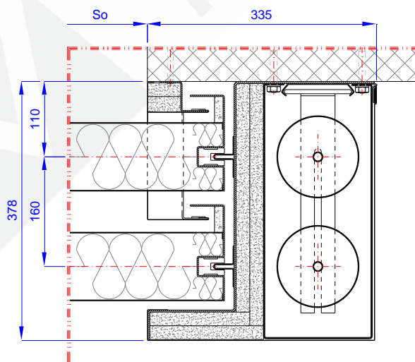
Fig. 3 – Detail B from Fig. 1
