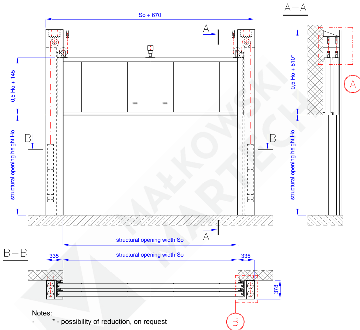
Fig. 1 – Fire protection vertically sliding telescopic door MARC-Ot EI120
