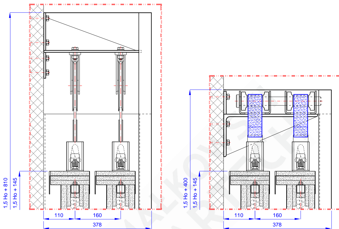
Fig. 2 – Detail A from Fig. 1 – variant with the cables on the left and with the belts on the right side
