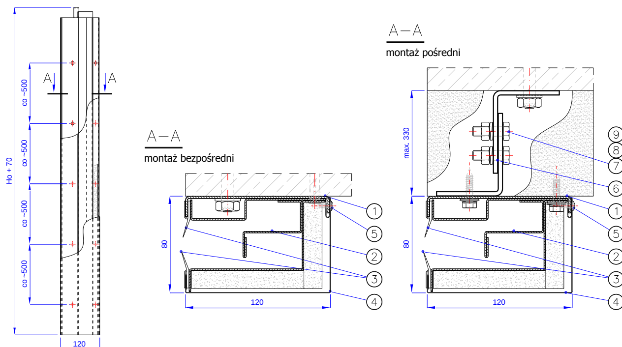
Rys. 9 - MARC-Ok60-01.04.00 [Prowadnica]
