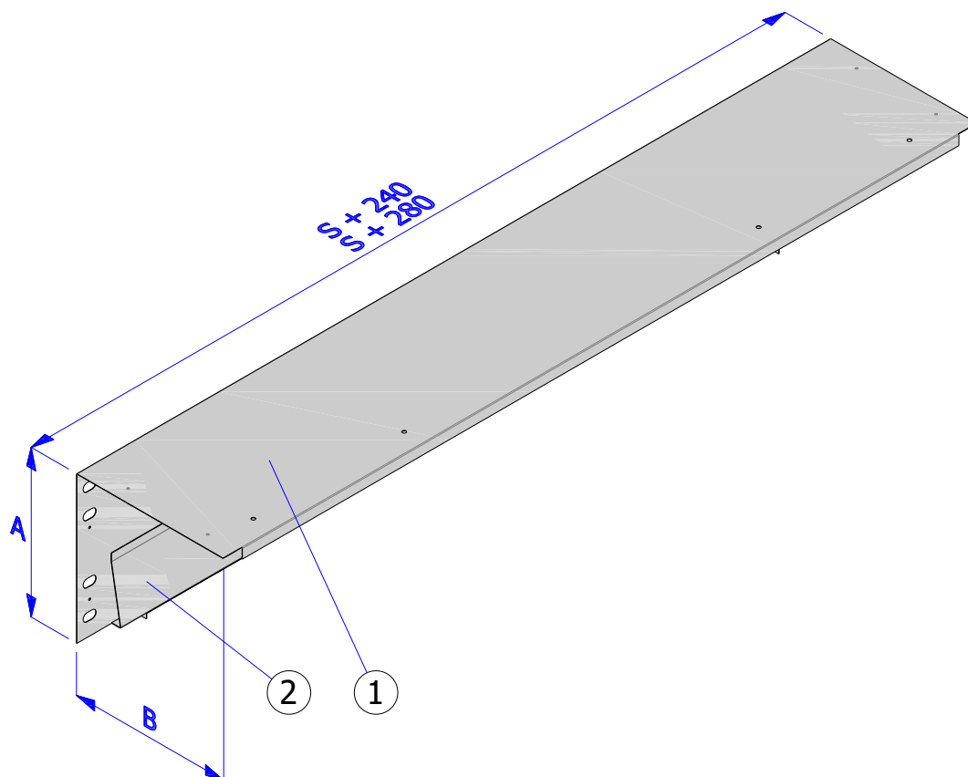
Rys. 12 - ISOiK-Ok60-01.12 [Ostona tylna]
