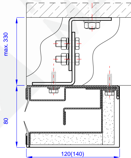
Fig. 3 – Fire protection curtain door MARC-Ok EI60, mixed mounting - no lintel and reveal on the right side
