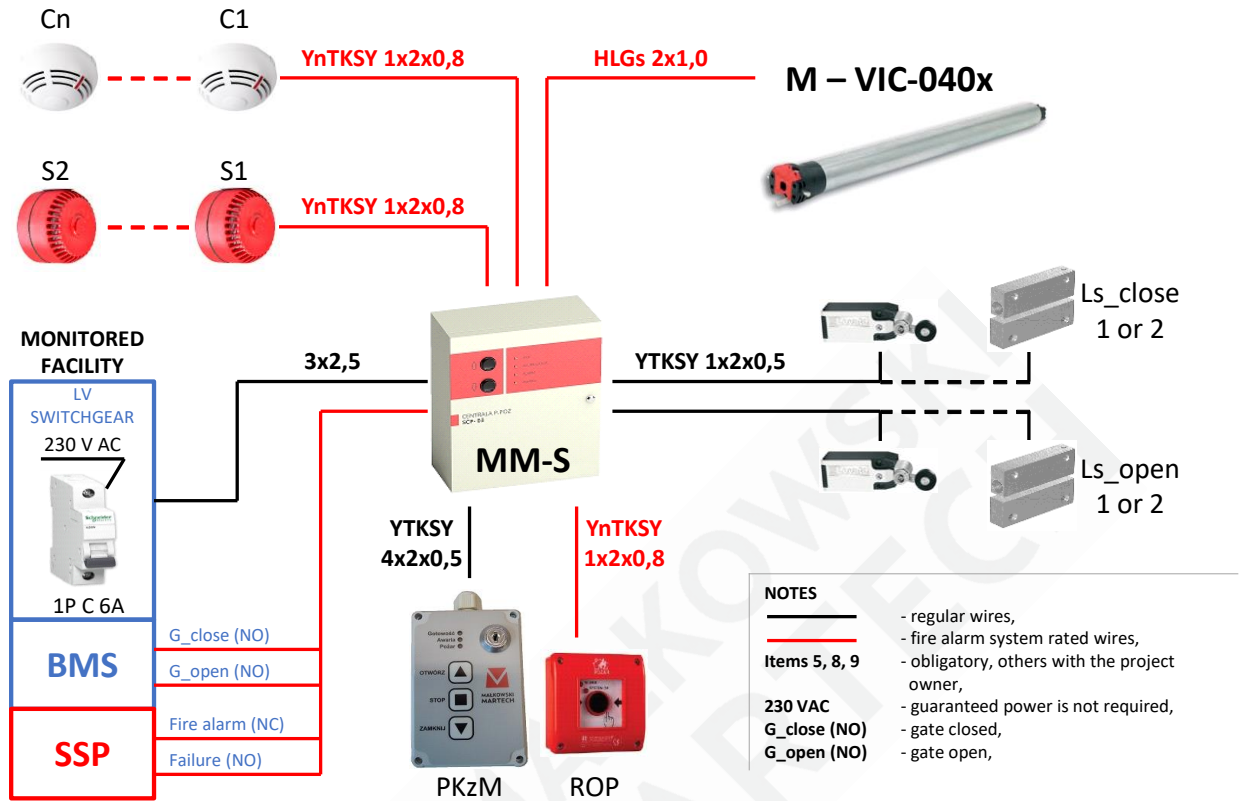
Fig. 5 – MARC-Ok control system with internally-mounted 24 V DC drive unit
