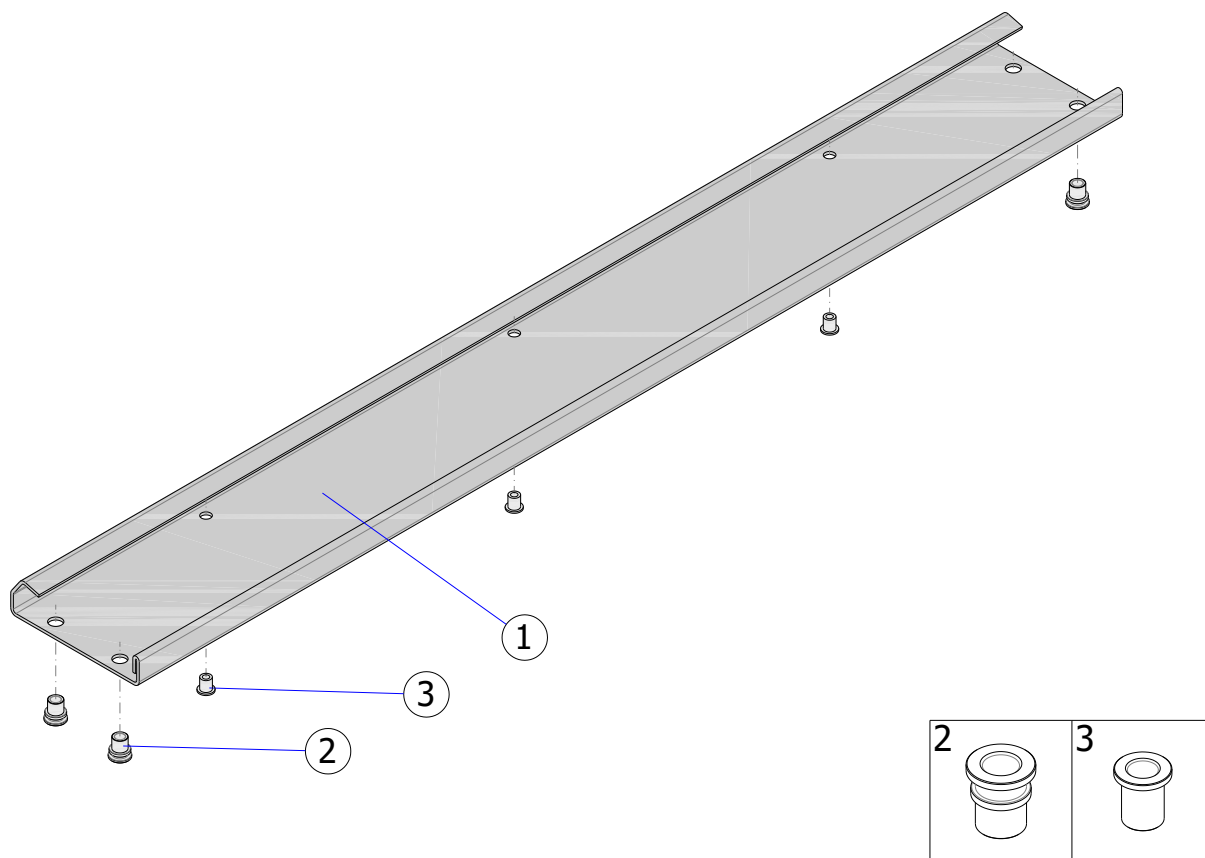
Fig. 26 - ISOiK-Ok60-01.26 [push bar]
