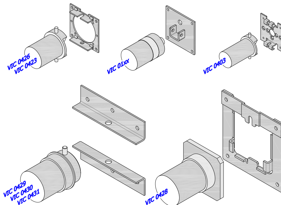
Fig. 9 - ISOiK-Ok60-01.09 [handles for individual internal drives]
