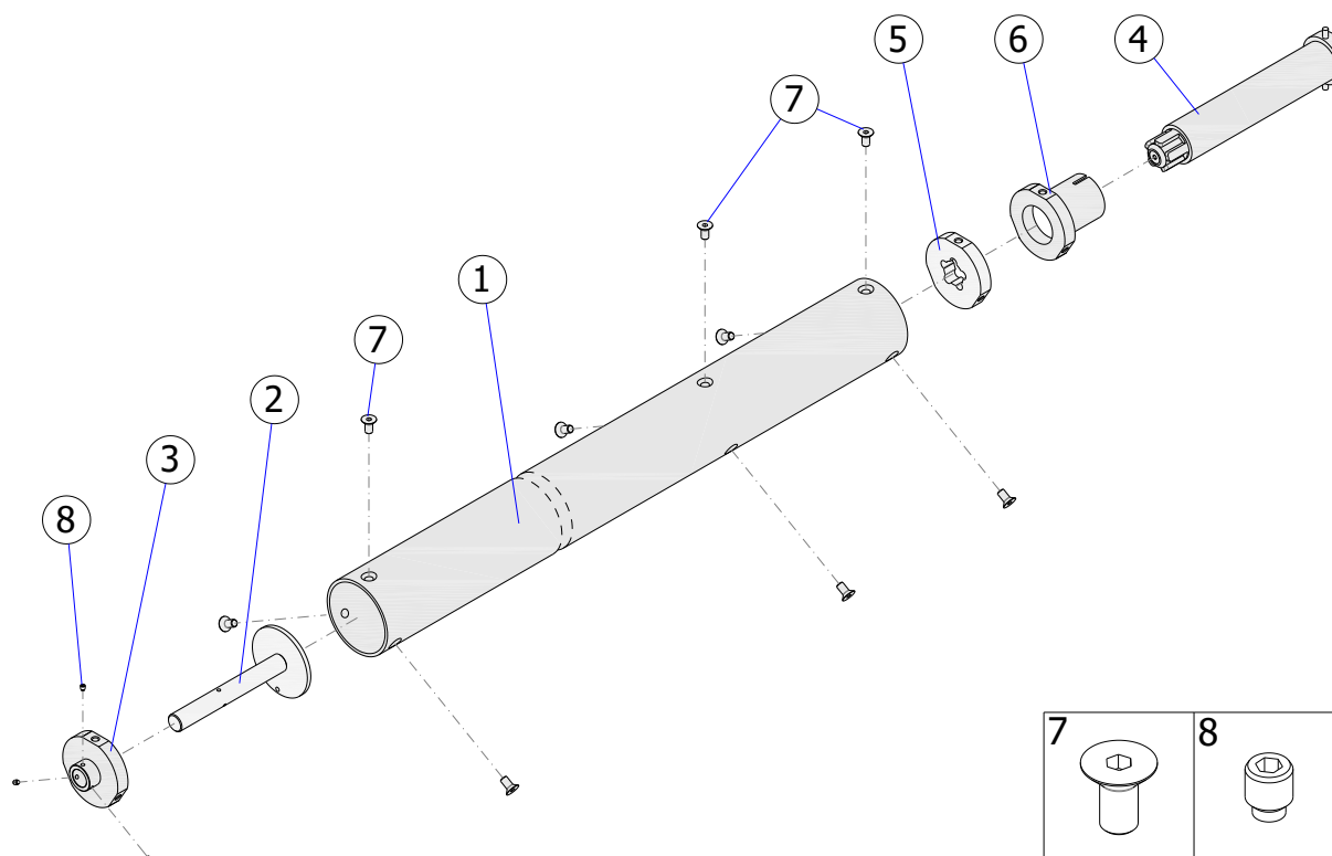
Fig. 19 – ISOiK-Ok60-01.19 [winding shaft with internal drive]
