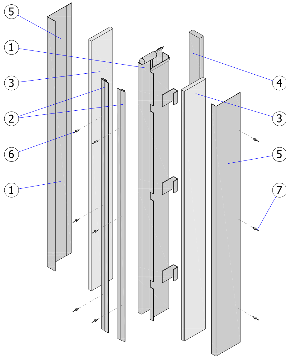
Fig. 22 – ISOiK-Ok60-01.22 [guide-rail – corridor-mounted version]
