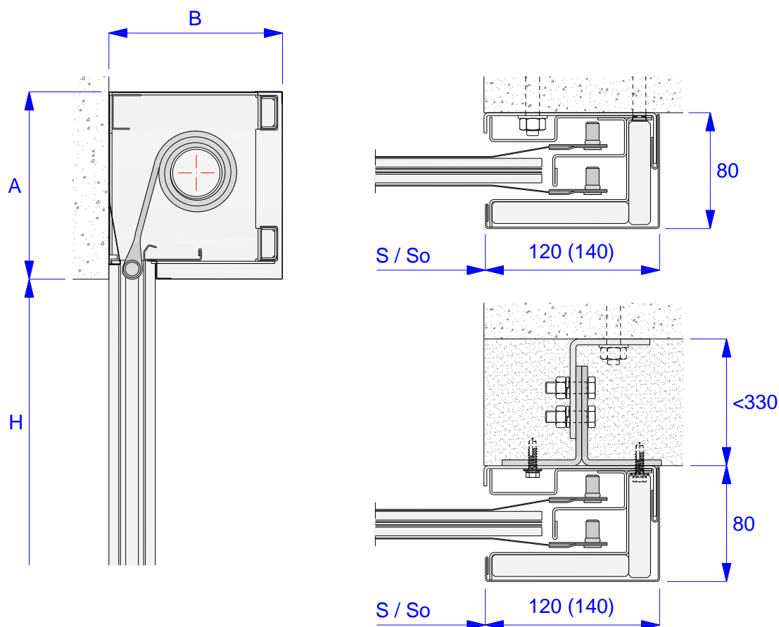
Fig. 3 - ISOiK-Ok60-01.03 MARC-Ok + EI60 fire protection curtain door – wall-mounted
