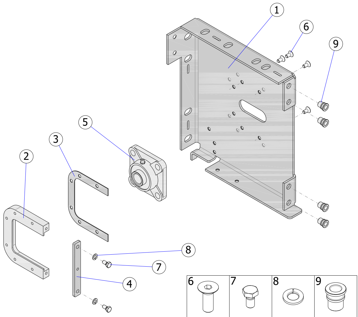
Fig. 24 – ISOiK-Ok60-01.24 [shaft bracket - passive side]
