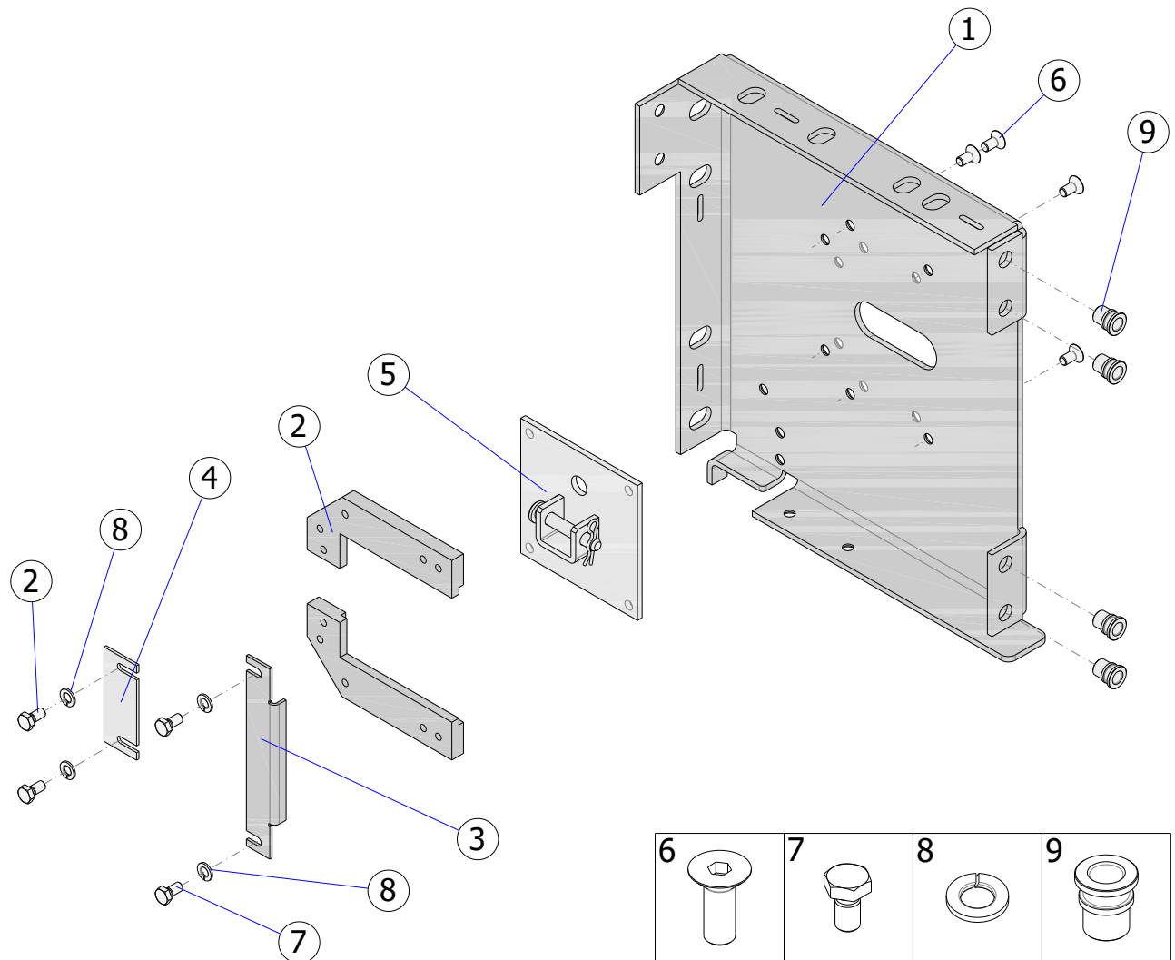
Fig. 23 – ISOiK-Ok60-01.23 [shaft bracket - drive side]
