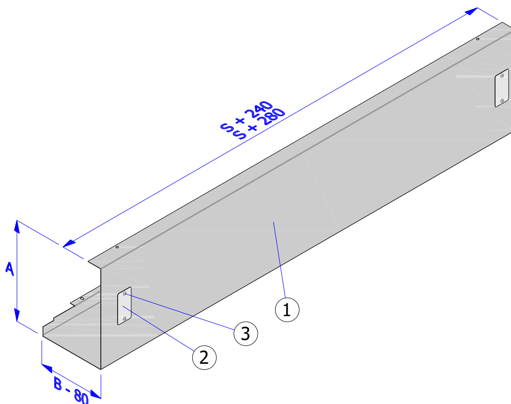
Fig. 13 - ISOiK-Ok60-01.13 [front guard]
