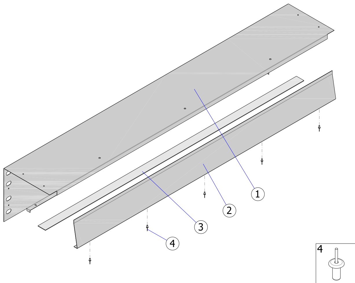
Fig. 27 - ISOiK-Ok60-01.27 [rear guard]
