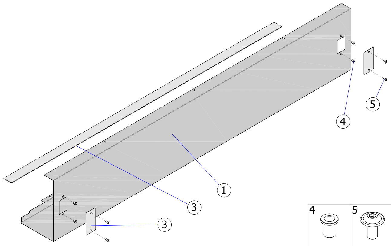
Fig. 28 - ISOiK-Ok60-01.28 [front guard]
