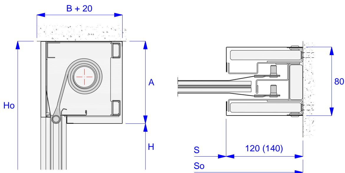
Fig. 4 - ISOiK-Ok60-01.04 Fire curtain door type MARC-Ok + EI60 - corridor (recessed) installation S - width of passage opening, So - width of door opening / wall opening
