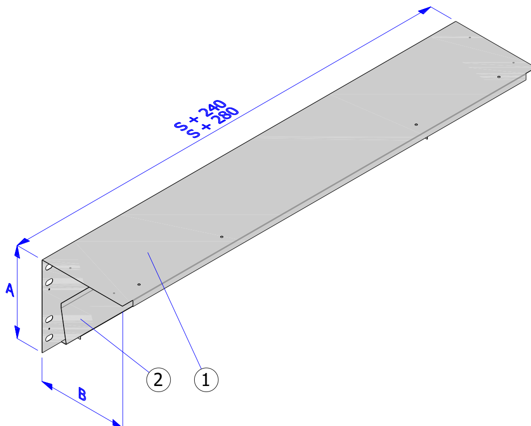
Fig. 12 - ISOiK-Ok60-01.12 [rear guard]
