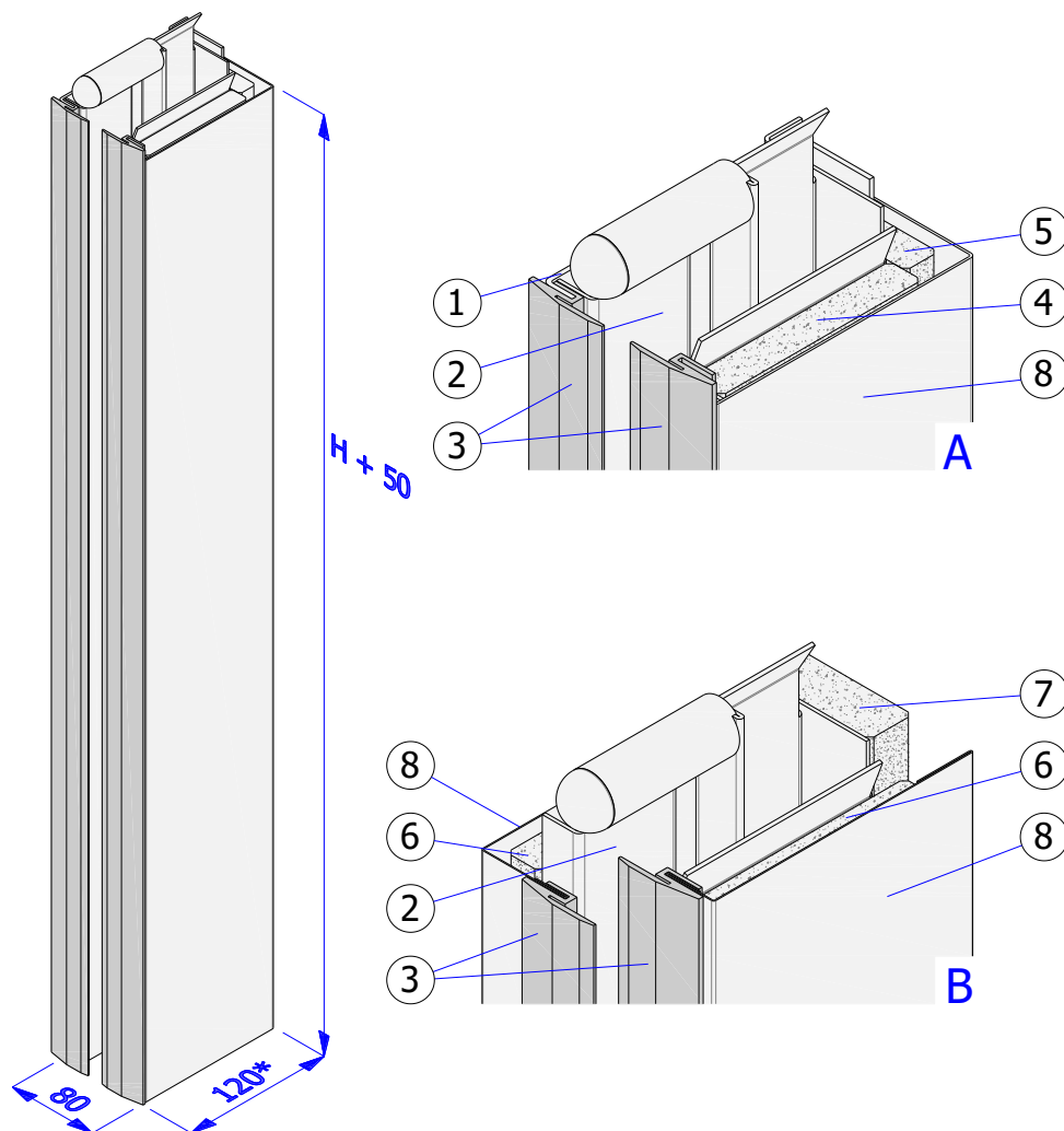
Fig. 7 - ISOiK-Ok60-01.07 [Guide, A - fire version, wall-mounted, B - fire version, corridor].
