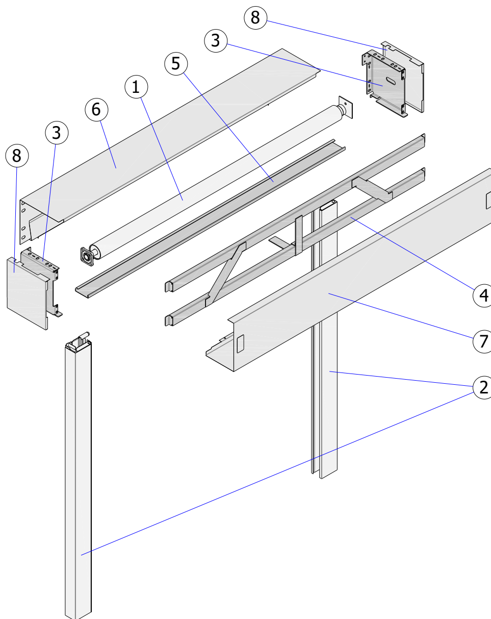
Fig. 2 - ISOiK-Ok60-01.02 Fire curtain gate MARC-Ok + EI60 with internal actuation
