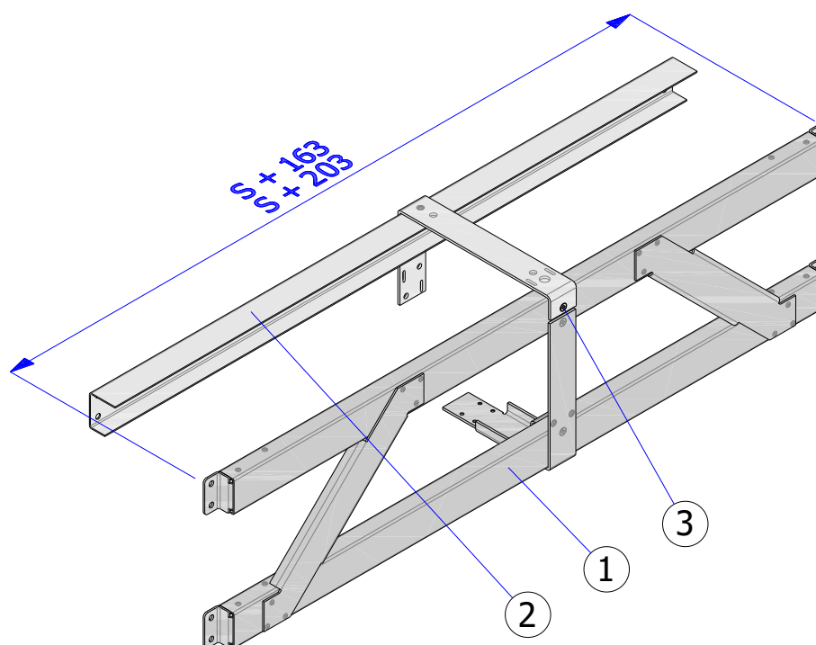
Fig. 10 - ISOiK-Ok30-01.10 [structural lattice with wall-mounted channel section]
