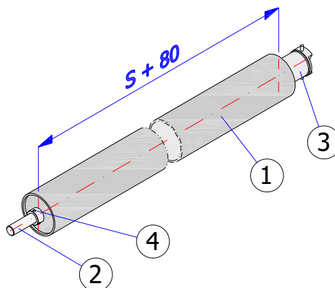
Fig. 5 – ISOiK-Ok30-01.05 [winding shaft with internal drive]
