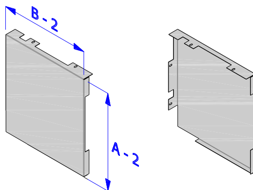
Fig. 14 - ISOiK-Ok30-01.14 [side guard]
