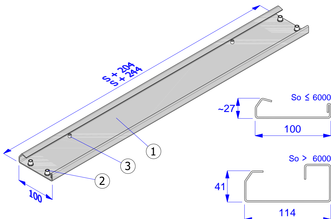
Fig. 11 - ISOiK-Ok30-01.11 [push bar]
