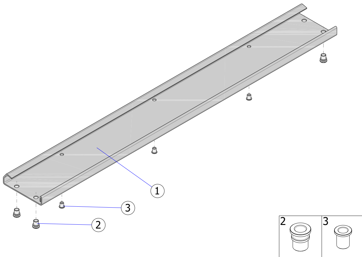
Fig. 26 - ISOiK-Ok30-01.26 [push bar]
