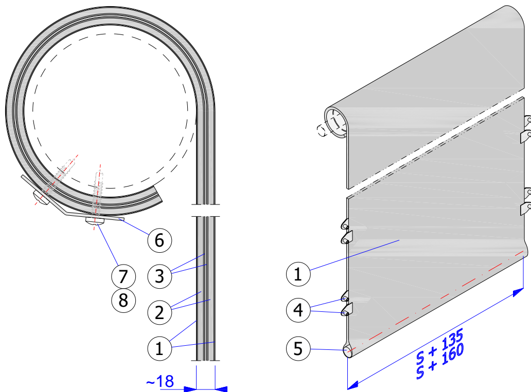
Fig. 6 - ISOiK-Ok30-01.06 [gate sheet]
