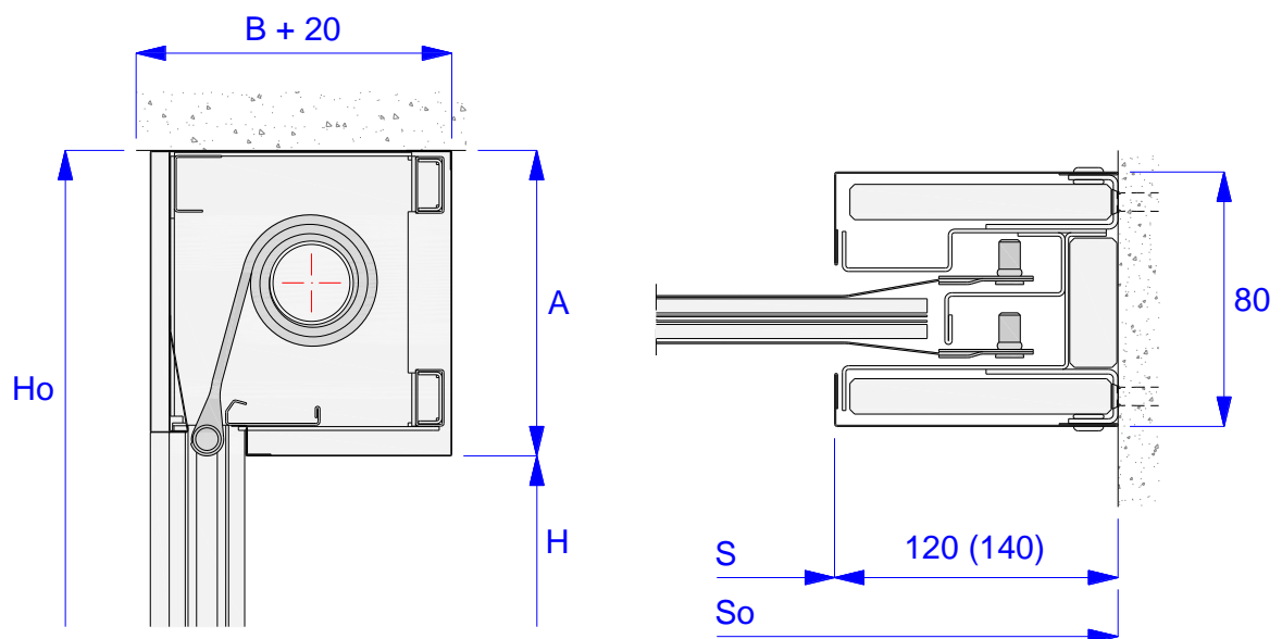
Fig. 4 - ISOiK-Ok30-01.04 Fire curtain door type MARC-Ok + EI30 - corridor (recessed) installation S - width of passage opening, So - width of door opening / wall opening
