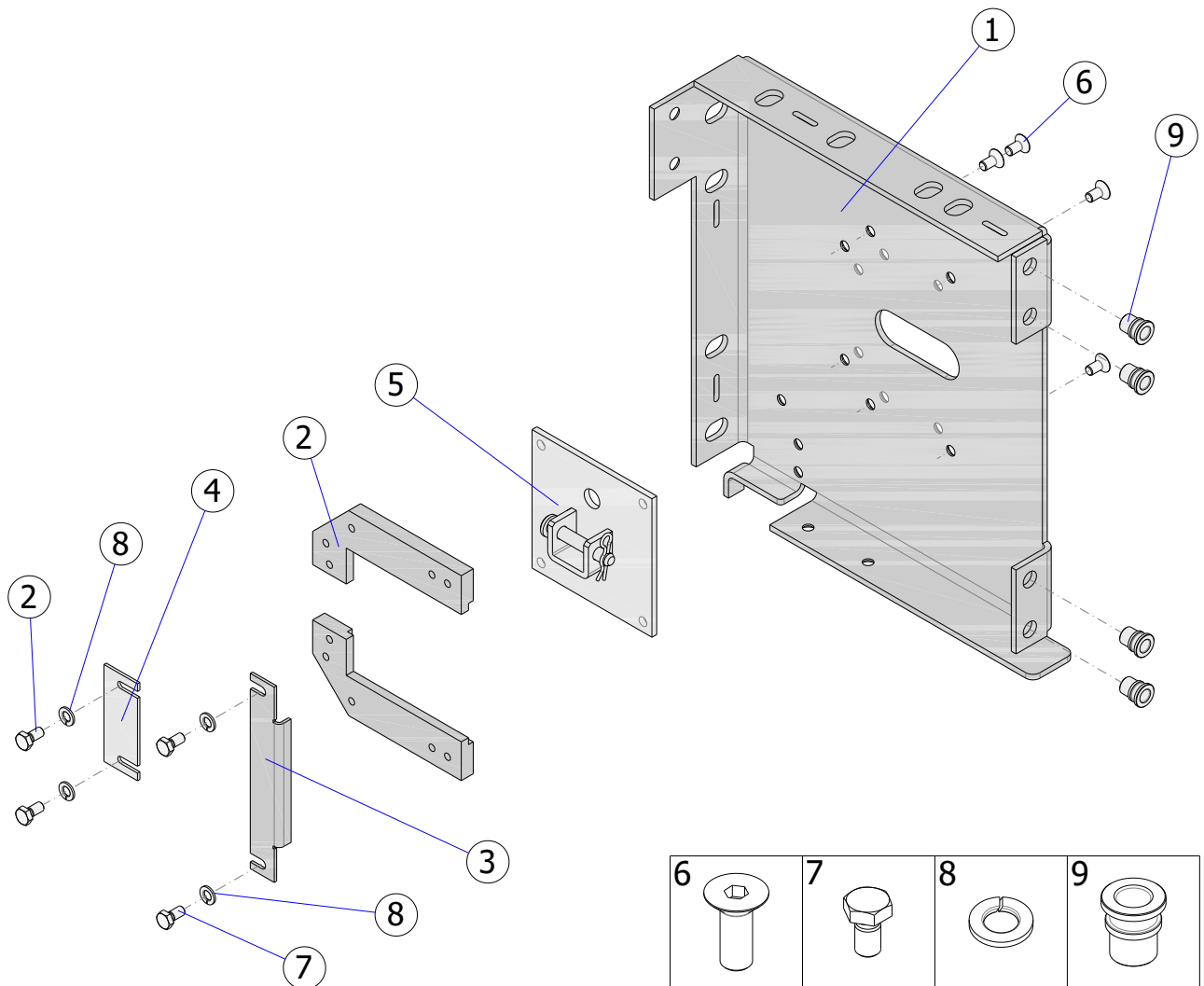
Fig. 23 – ISOiK-Ok30-01.23 [shaft bracket - drive side]
