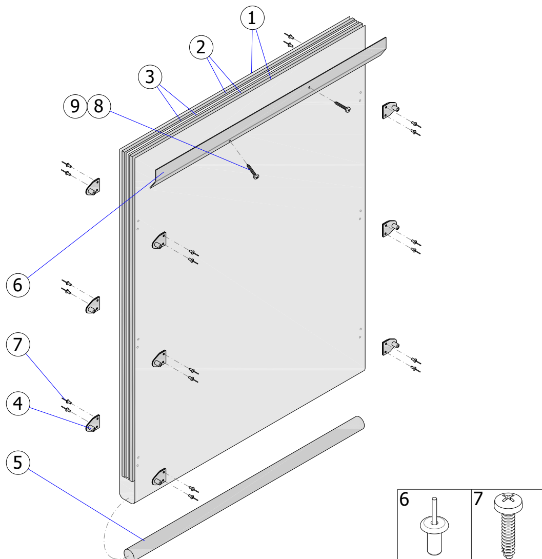
Fig. 20 - ISOiK-Ok30-01.20 [gate sheet]
