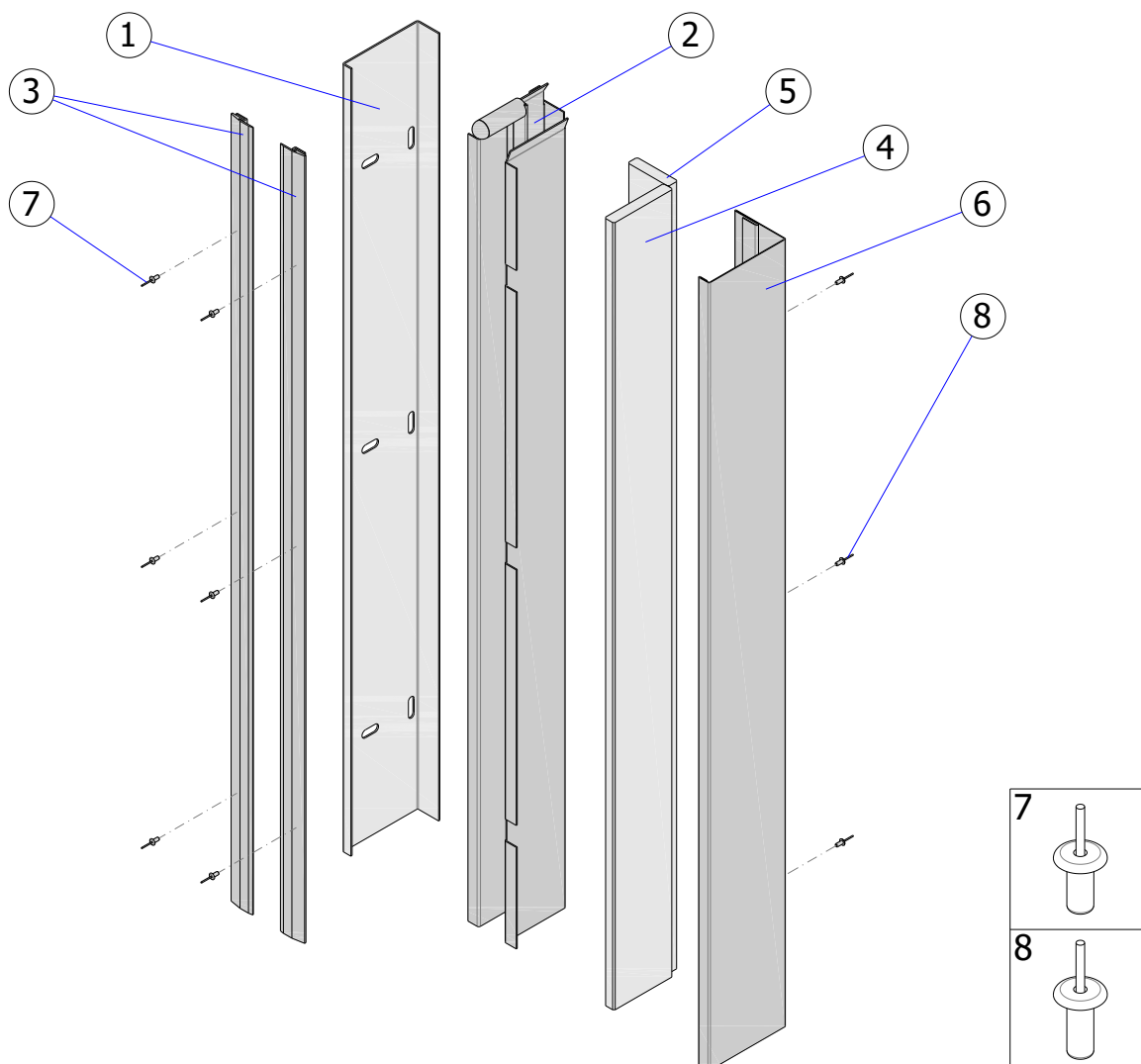
Fig. 21 - ISOiK-Ok30-01.21 [Guide rail - wall-mounted version].
