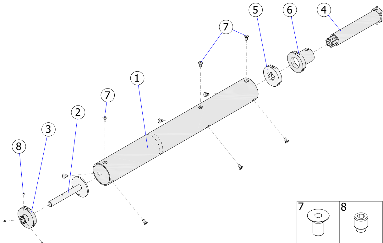
Fig. 19 – ISOiK-Ok30-01.19 [winding shaft with internal drive]
