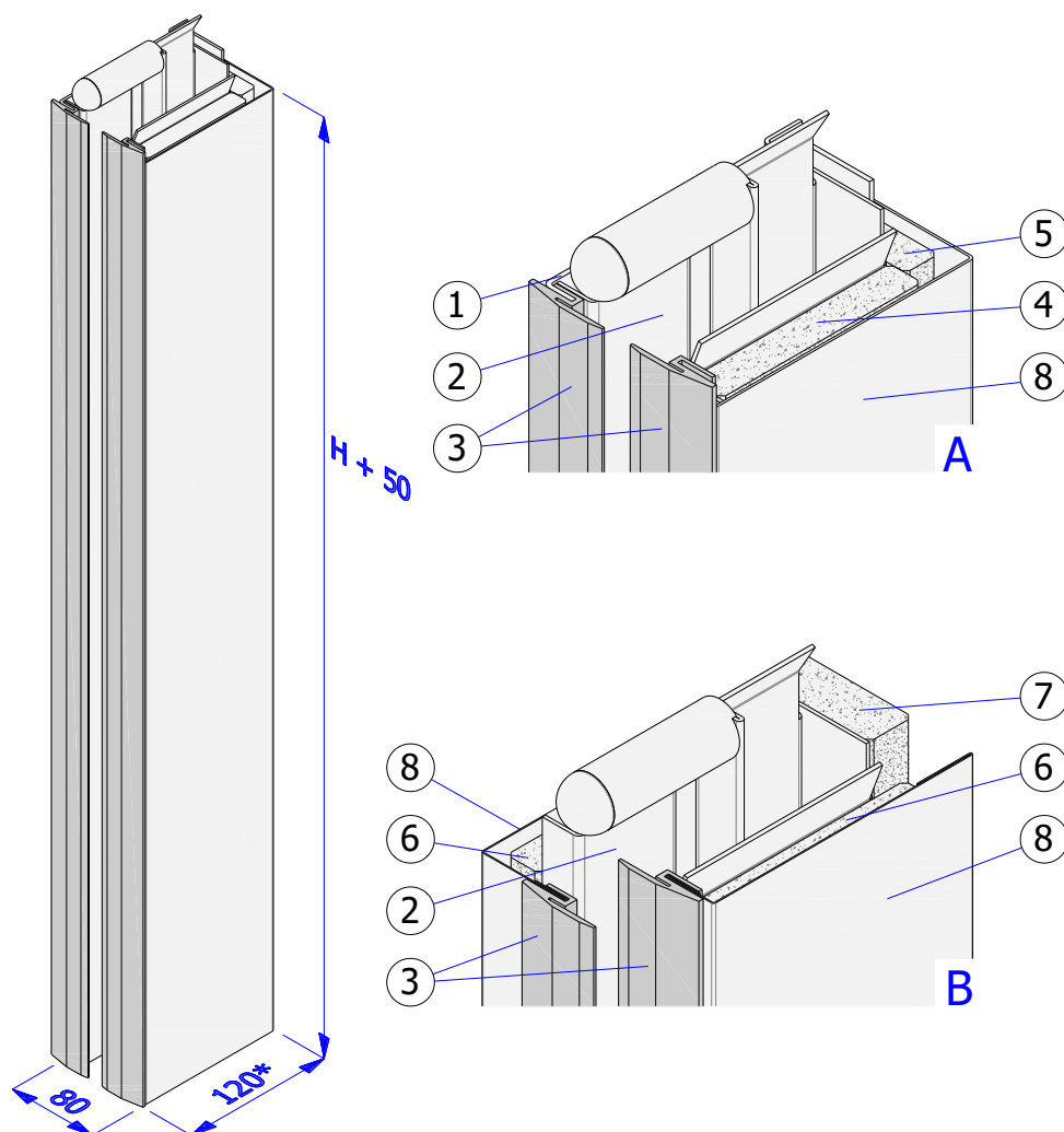
Fig. 7 - ISOiK-Ok30-01.07 [Guide, A - fire version, wall-mounted, B - fire version, corridor].
