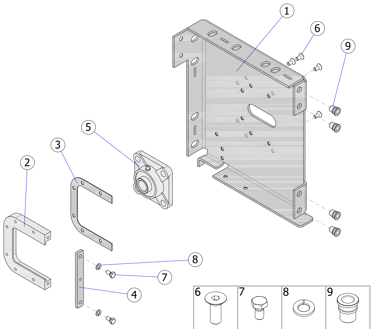
Fig. 24 – ISOiK-Ok30-01.24 [shaft bracket - passive side]
