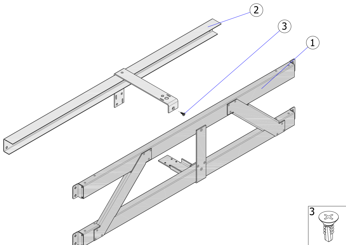
Fig. 25 - ISOiK-Ok30-01.25 [structural lattice with wall-mounted channel section]
