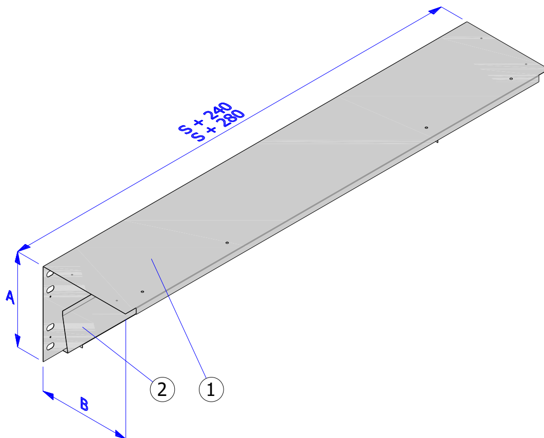
Fig. 12 - ISOiK-Ok30-01.12 [rear guard]
