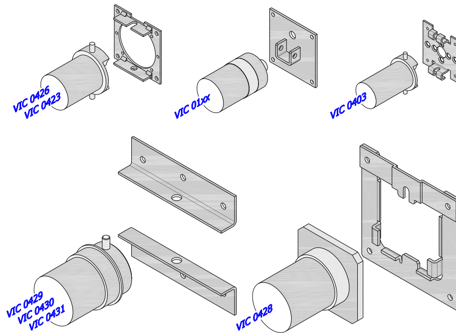
Fig. 9 - ISOiK-Ok30-01.09 [handles for individual internal drives]
