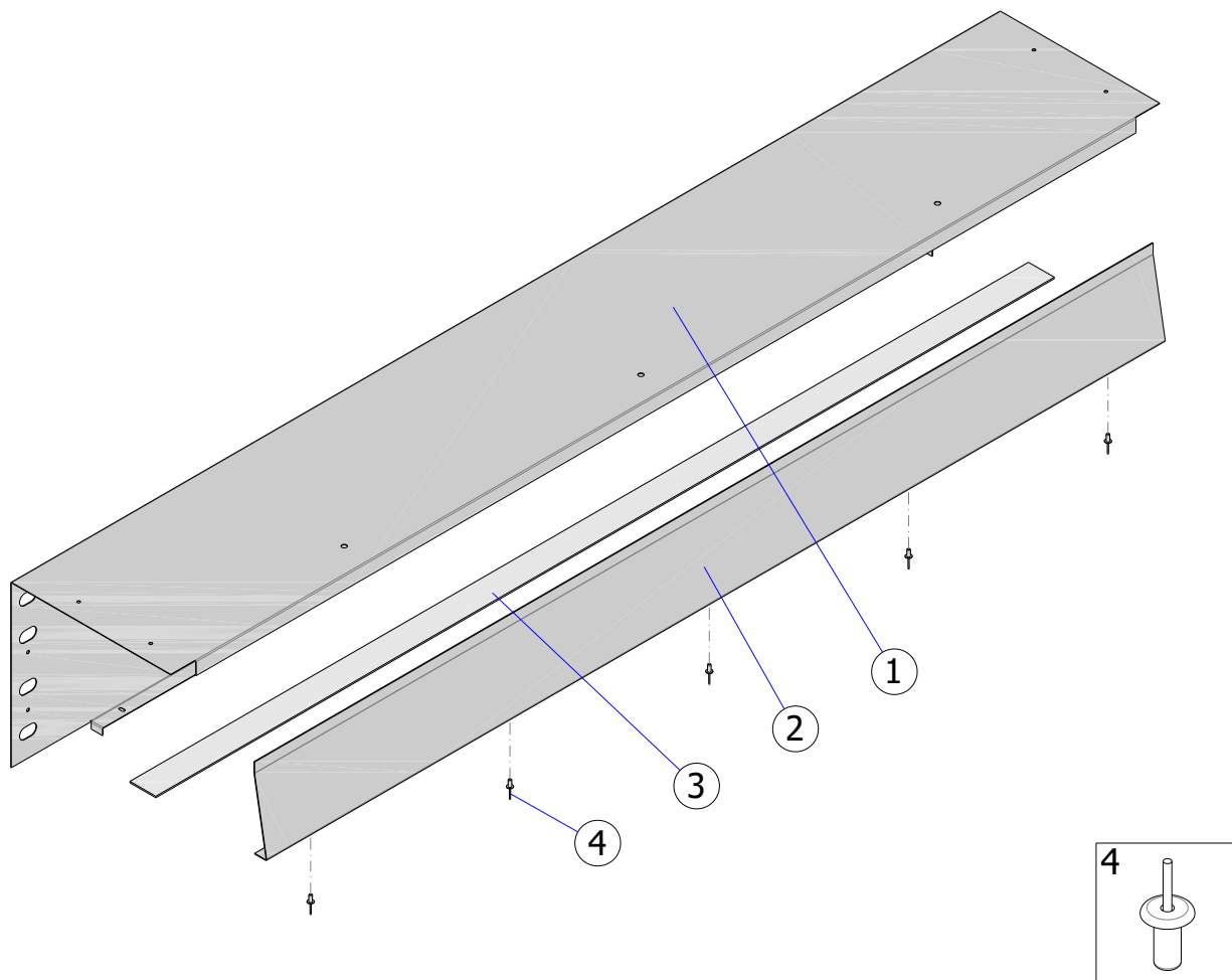
Fig. 27 - ISOiK-Ok30-01.27 [rear guard]
