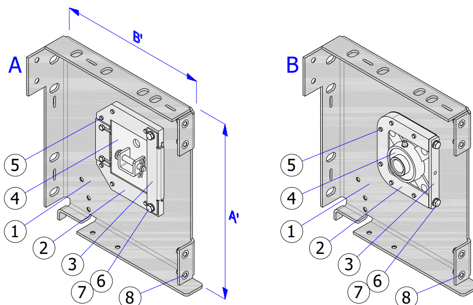
Fig. 8 - ISOiK-Ok30-01.08 [Shaft bracket, A - drive side, B - passive side]
