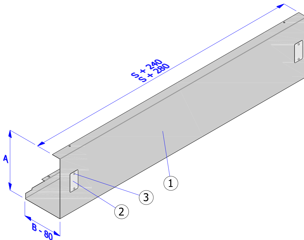
Fig. 13 - ISOiK-Ok30-01.13 [front guard] 1 – Guard profile, 2 – Inspection hole cap
